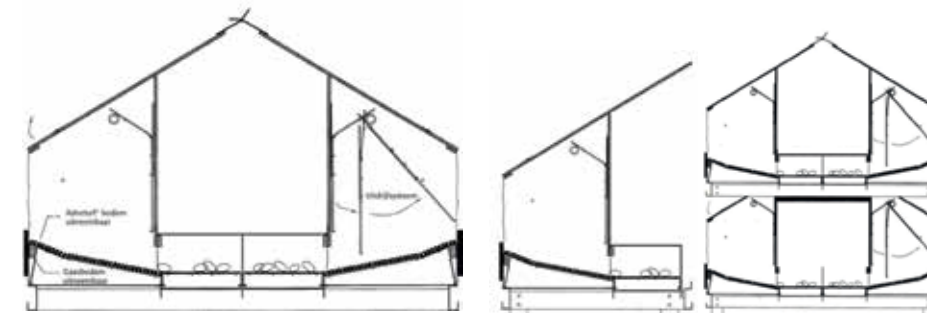
Cross-section of the standard configuration.
